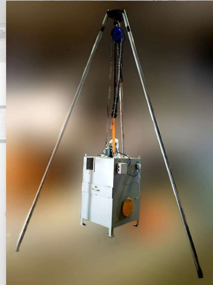
TRIPOD ASSEMBLY
