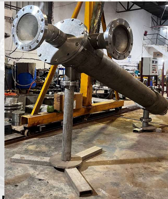
HYDRO CYCLONE SEPERATOR
