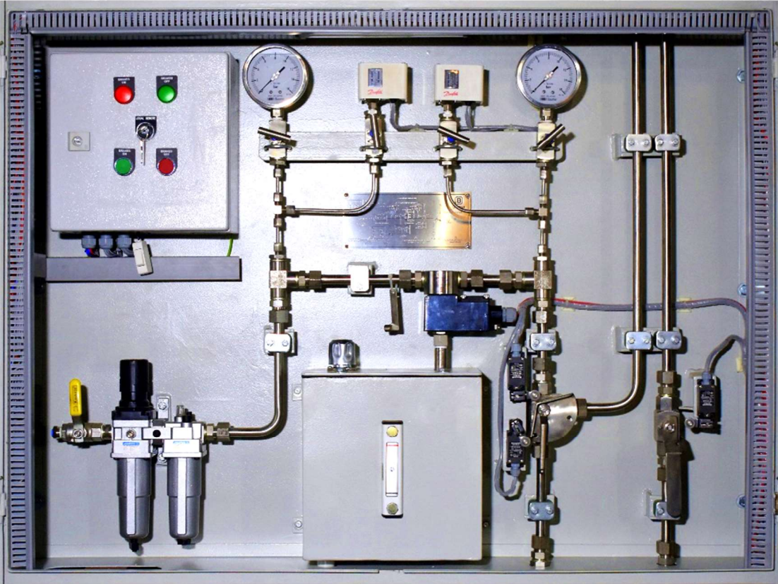
MECHANICAL CONTROL PANELS
